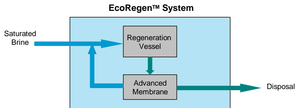
Figure 2: EcoRegen™ System Flow Diagram
