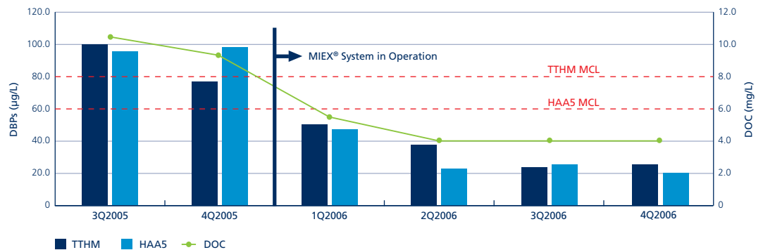
Figure 2: The DOC removal provided by the MIEX® System prior to microfiltration at Big Elk Meadows, Colorado has resulted in significant reductions in Trihalomethanes (THMs) and Haloacetic Acids (HAAs).
