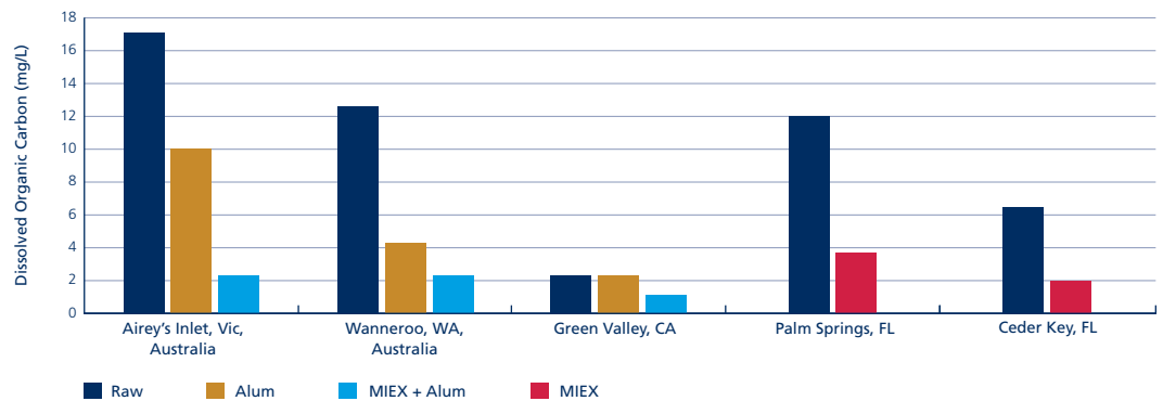
Figure 1: DOC reduction achieved with MIEX® treatment and coagulation at full-scale installations.
